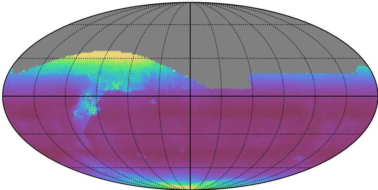
weather_cloudso14v3.4_10yrs All sky i band: Median airmass
