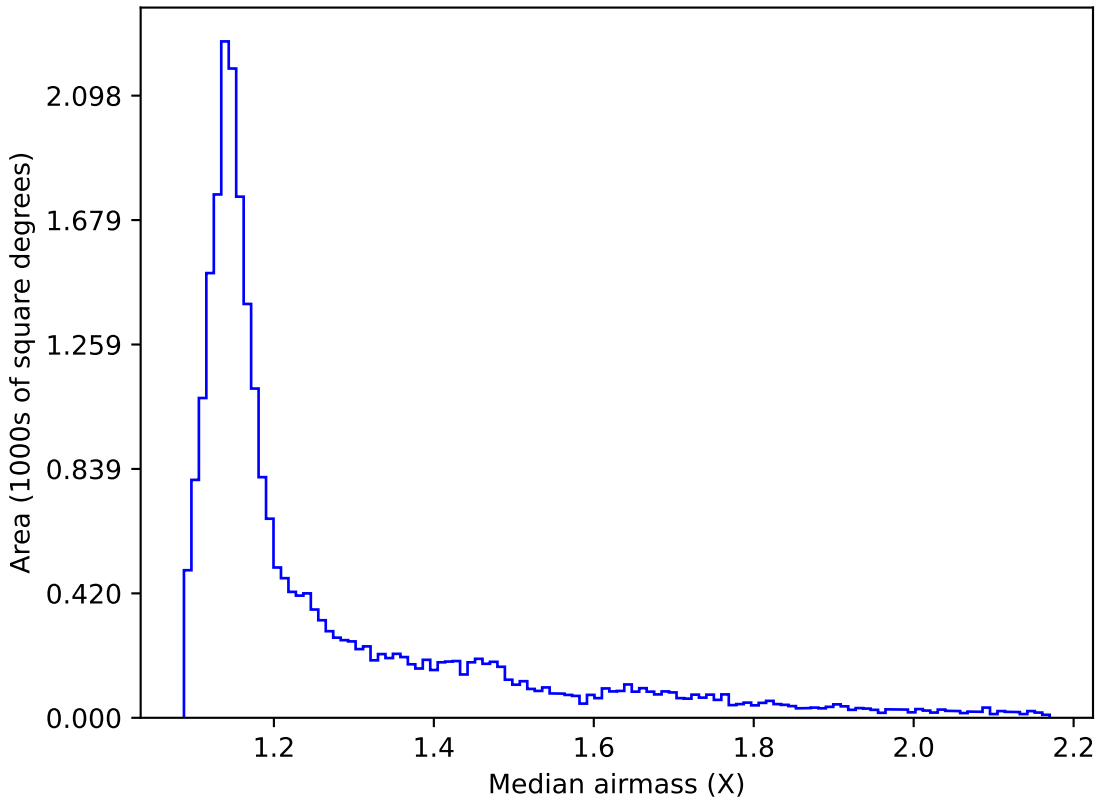
weather_cloudso14v3.4_10yrs All sky i band: Median airmass
