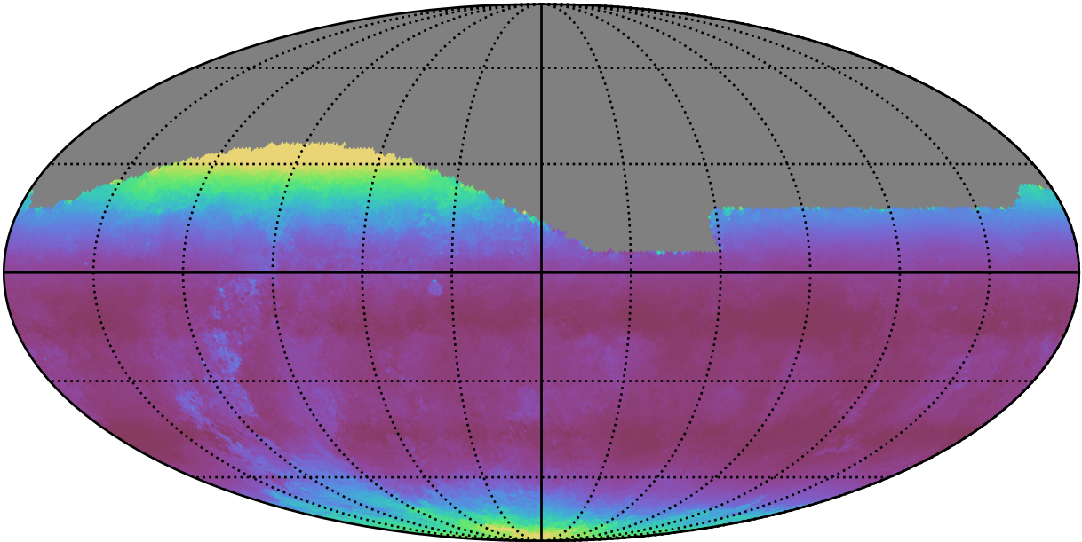
weather_cloudso14v3.4_10yrs All sky g band: Median airmass
