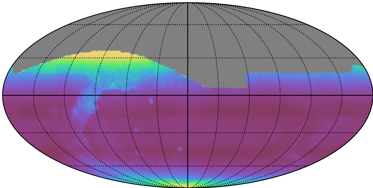
weather_cloudso14v3.4_10yrs All sky all bands: Median airmass
