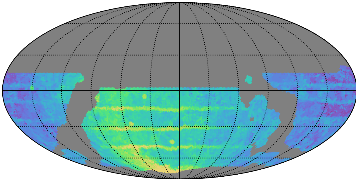
weather_cloudso14v3.4_10yrs WFD z band: Median Season Length
