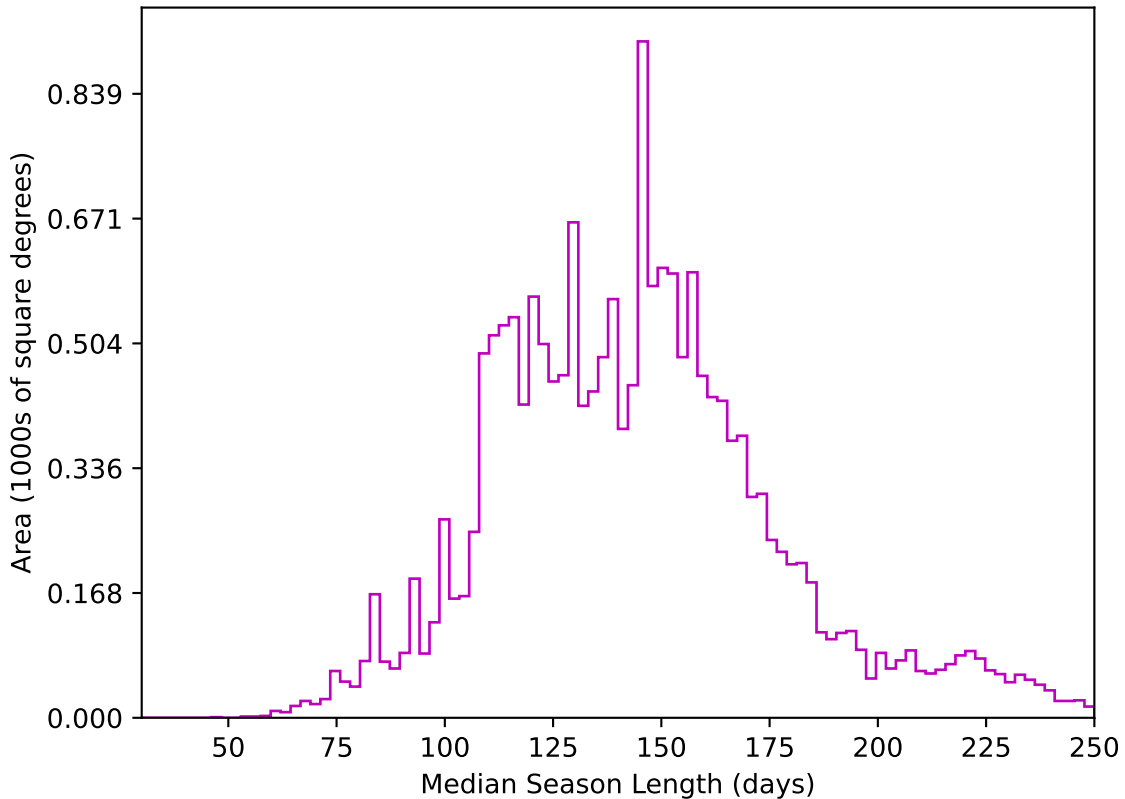
weather_cloudso14v3.4_10yrs WFD z band: Median Season Length
