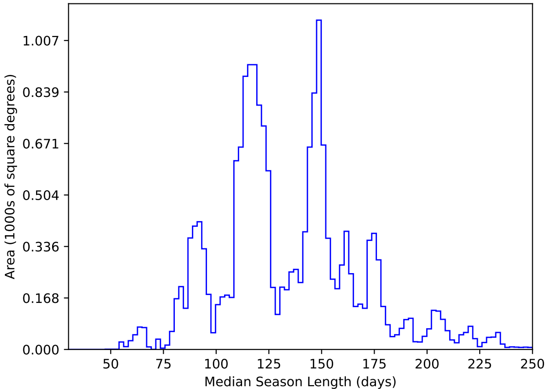
weather_cloudso14v3.4_10yrs WFD y band: Median Season Length
