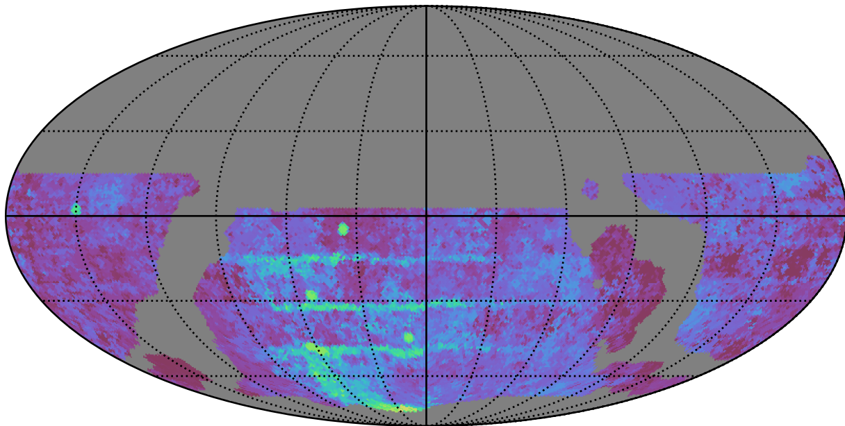
weather_cloudso14v3.4_10yrs WFD u band: Median Season Length
