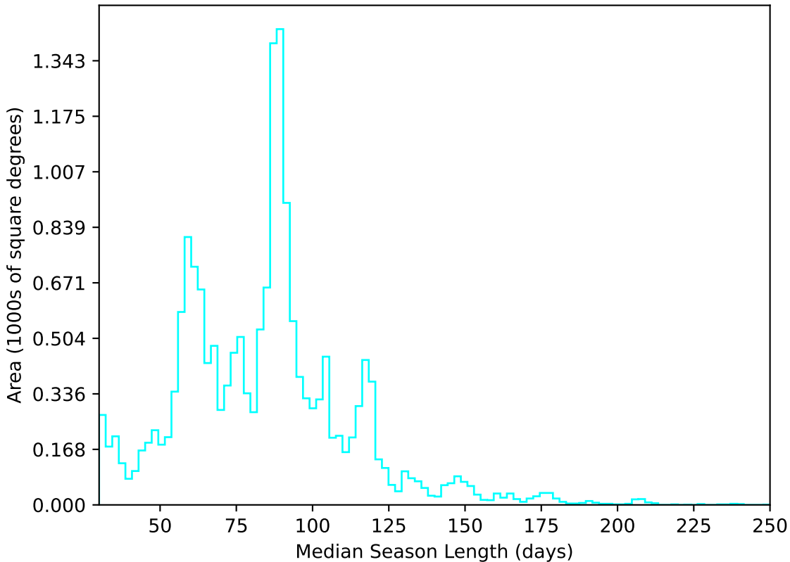
weather_cloudso14v3.4_10yrs WFD u band: Median Season Length
