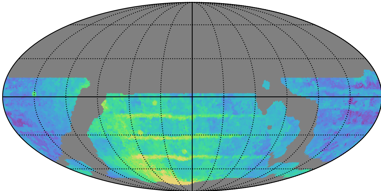
weather_cloudso14v3.4_10yrs WFD r band: Median Season Length
