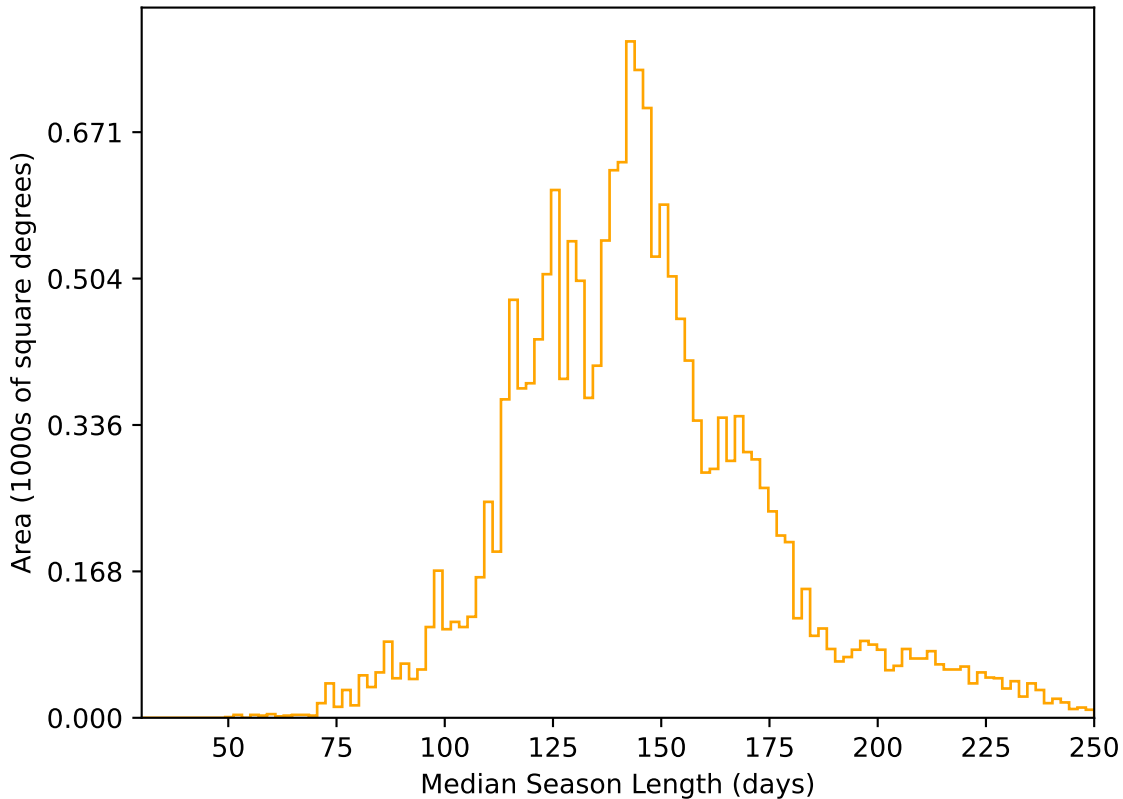
weather_cloudso14v3.4_10yrs WFD r band: Median Season Length
