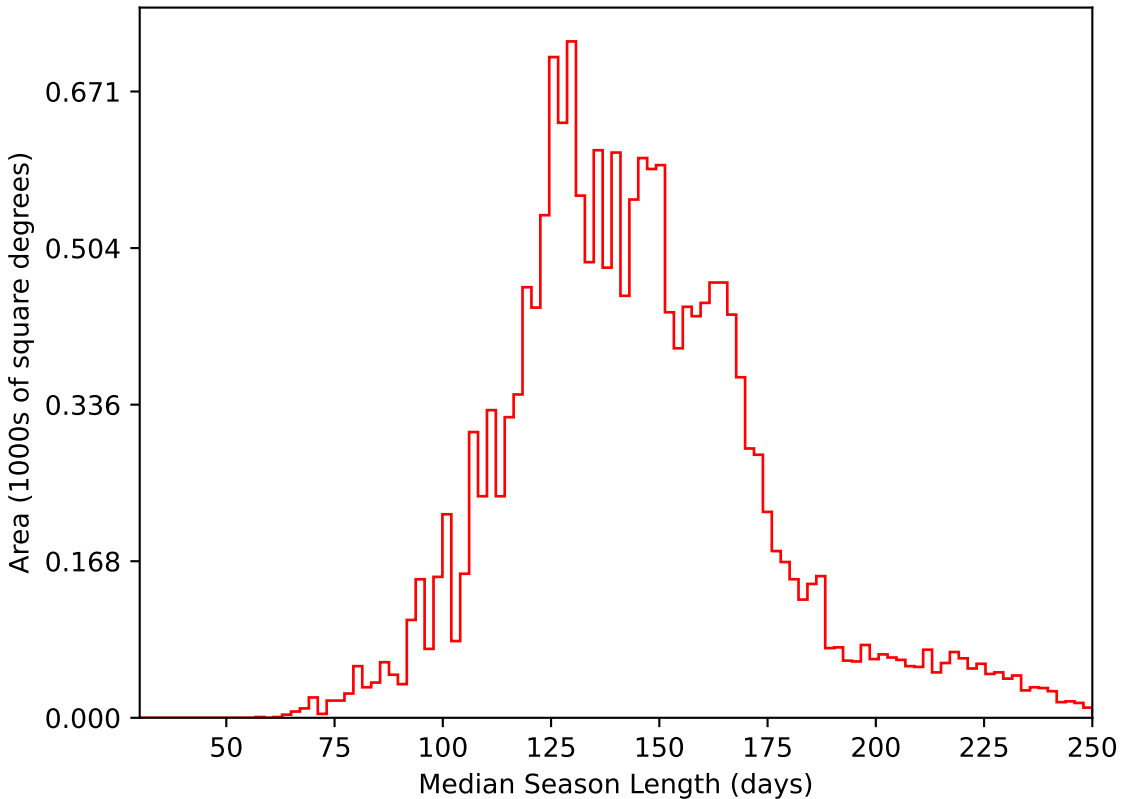
weather_cloudso14v3.4_10yrs WFD i band: Median Season Length
