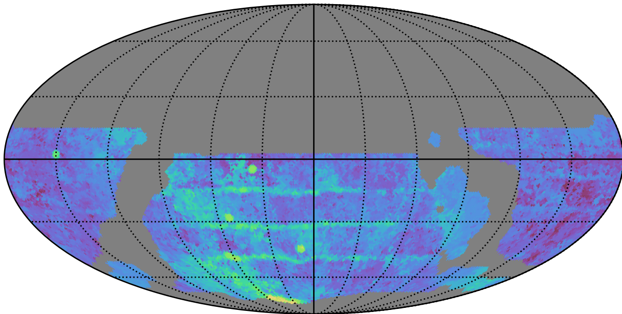
weather_cloudso14v3.4_10yrs WFD g band: Median Season Length
