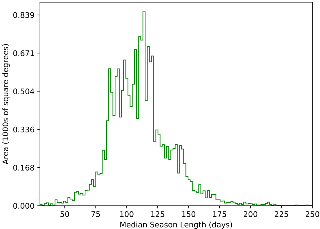
weather_cloudso14v3.4_10yrs WFD g band: Median Season Length
