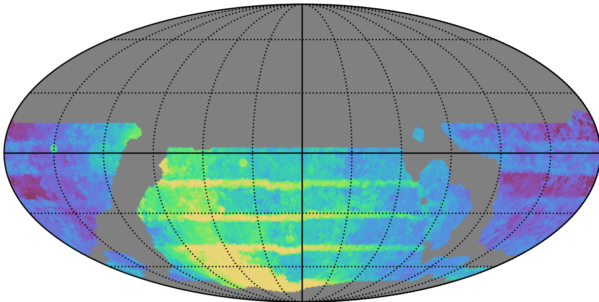
weather_cloudso14v3.4_10yrs WFD all bands: Median Season Length
