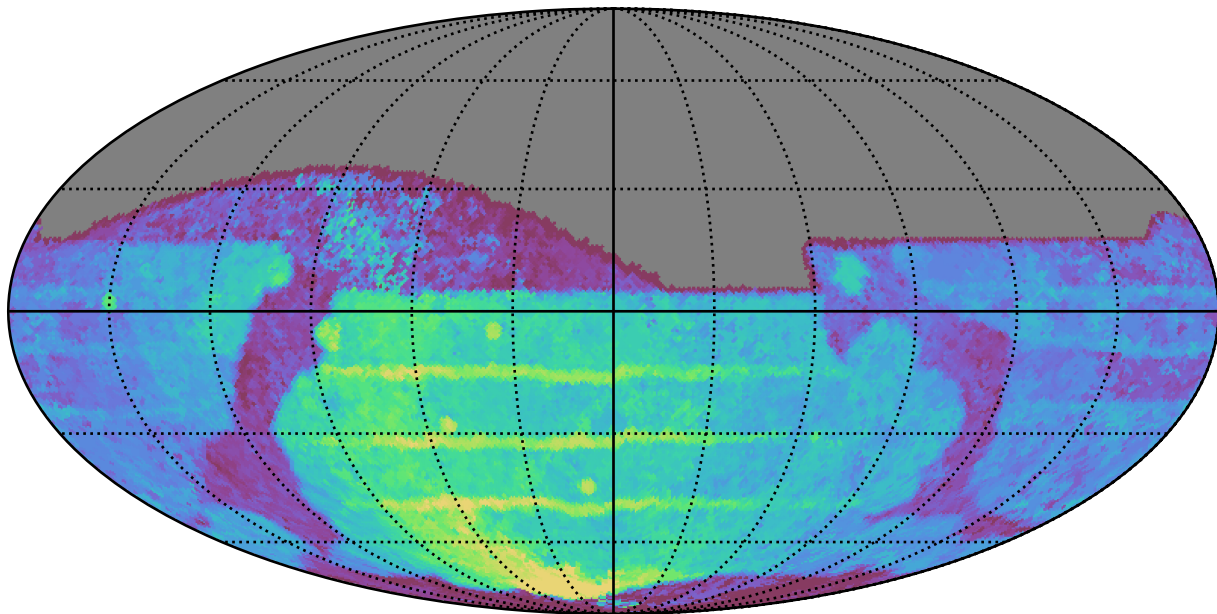
weather_cloudso14v3.4_10yrs All sky z band: Median Season Length
