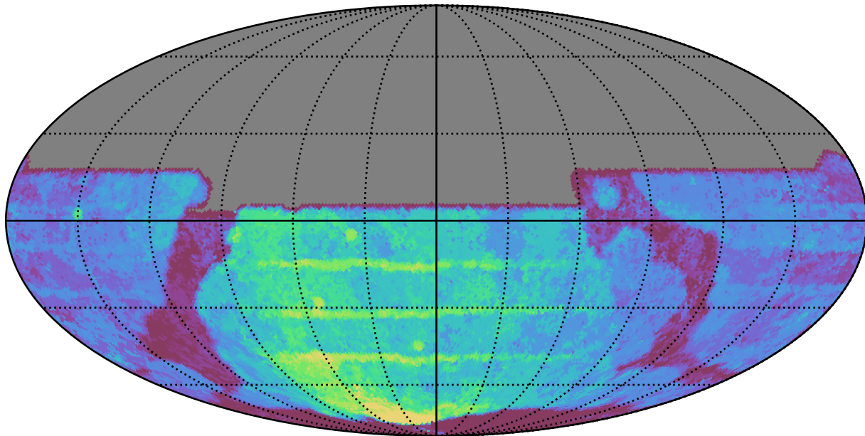
weather_cloudso14v3.4_10yrs All sky y band: Median Season Length
