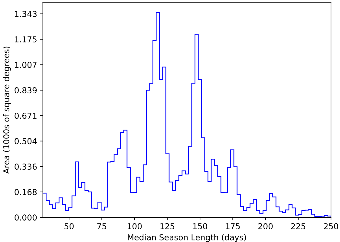
weather_cloudso14v3.4_10yrs All sky y band: Median Season Length
