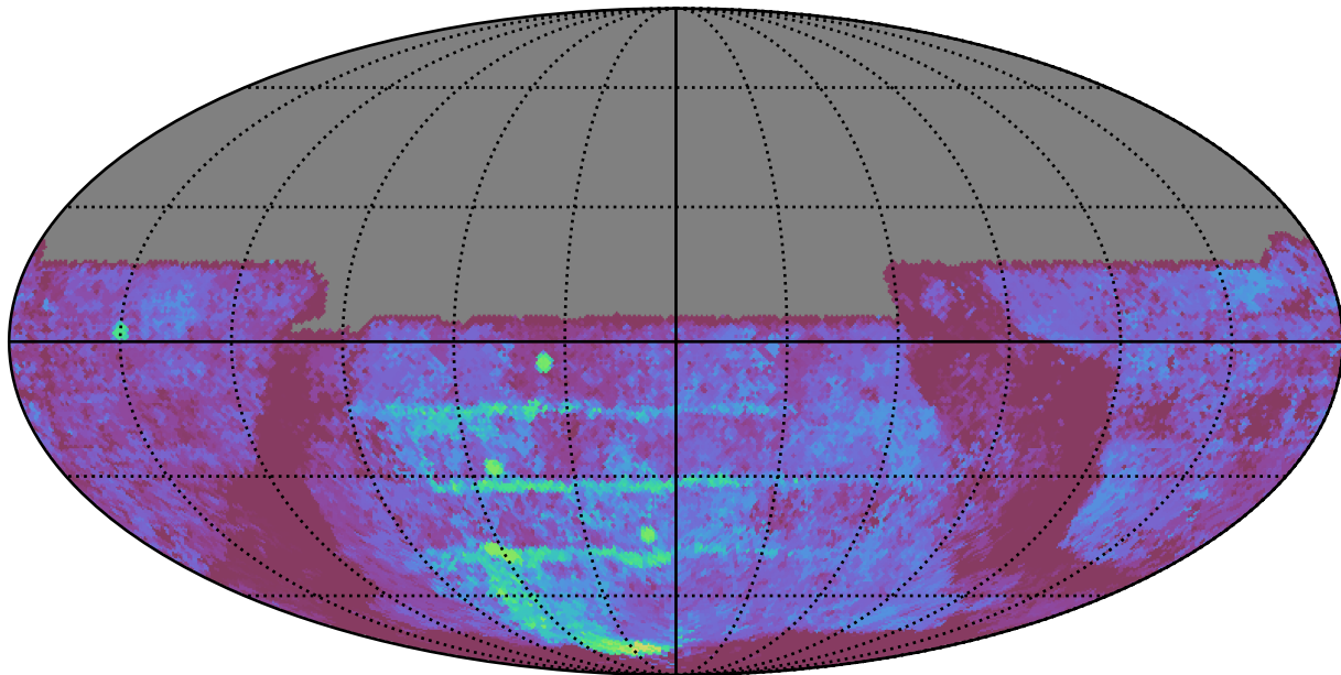
weather_cloudso14v3.4_10yrs All sky u band: Median Season Length
