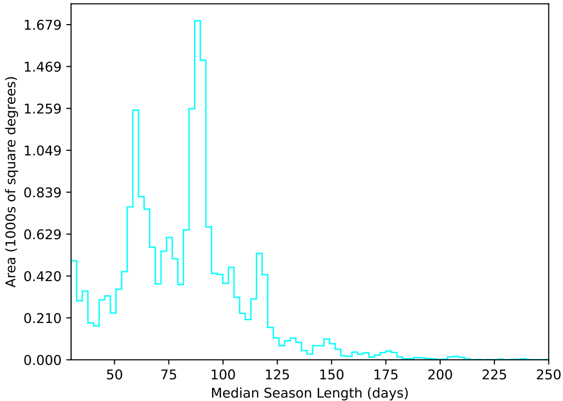
weather_cloudso14v3.4_10yrs All sky u band: Median Season Length
