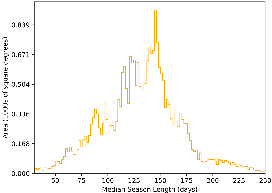
weather_cloudso14v3.4_10yrs All sky r band: Median Season Length
