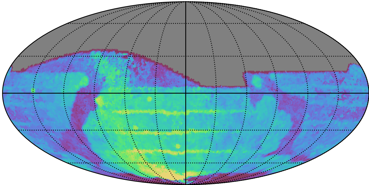
weather_cloudso14v3.4_10yrs All sky i band: Median Season Length
