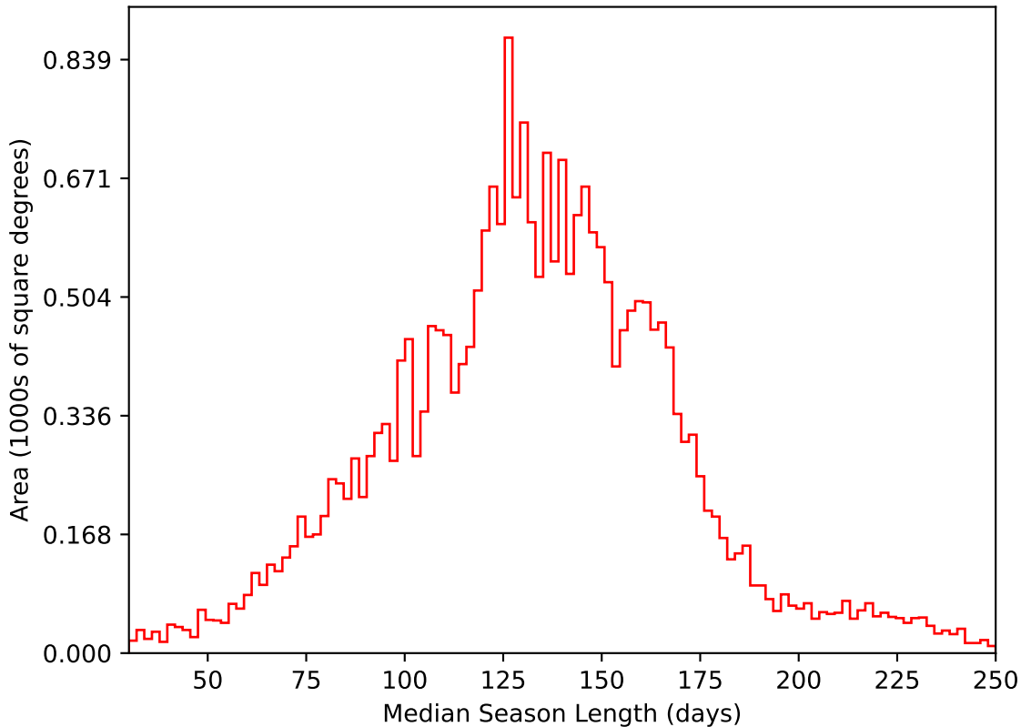
weather_cloudso14v3.4_10yrs All sky i band: Median Season Length
