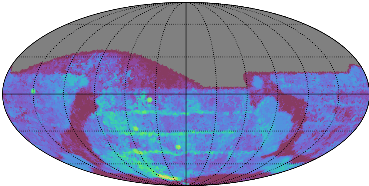
weather_cloudso14v3.4_10yrs All sky g band: Median Season Length
