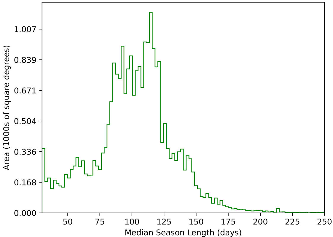
weather_cloudso14v3.4_10yrs All sky g band: Median Season Length
