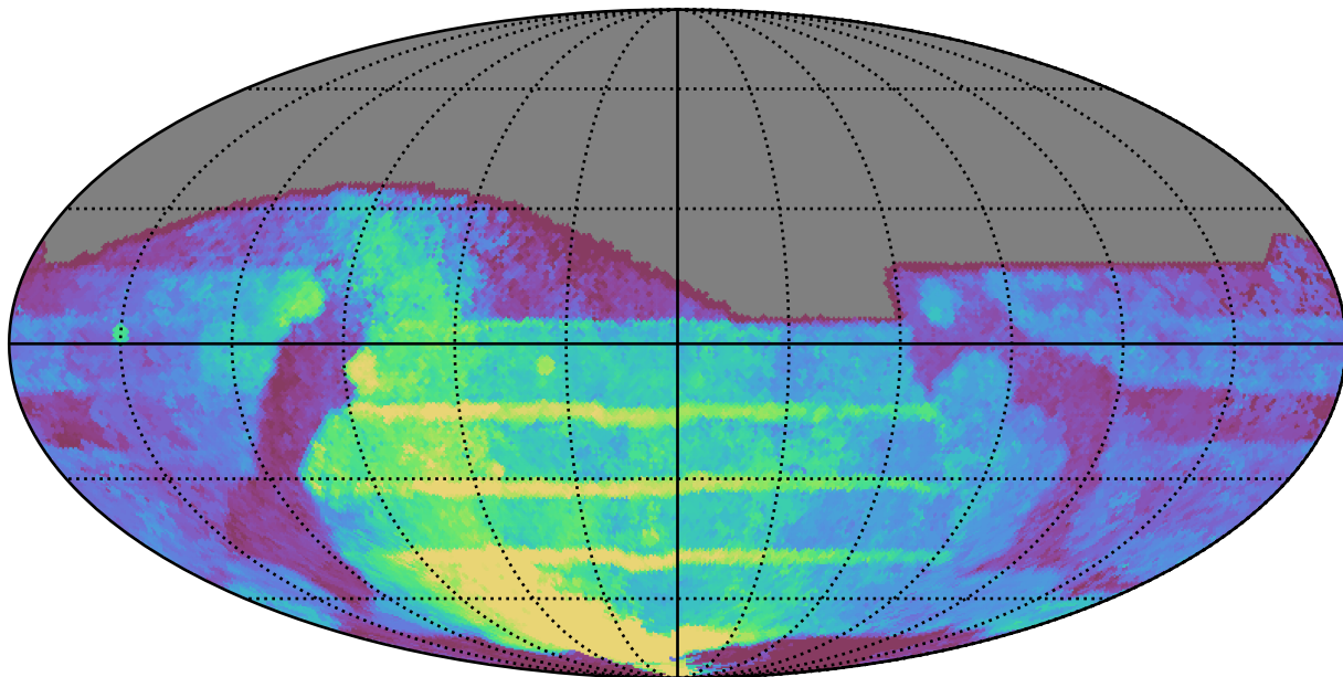
weather_cloudso14v3.4_10yrs All sky all bands: Median Season Length
