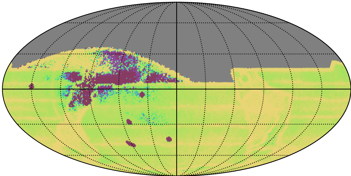
weather_cloudso14v3.4_10yrs All sky: Median Intra-Night Gap
