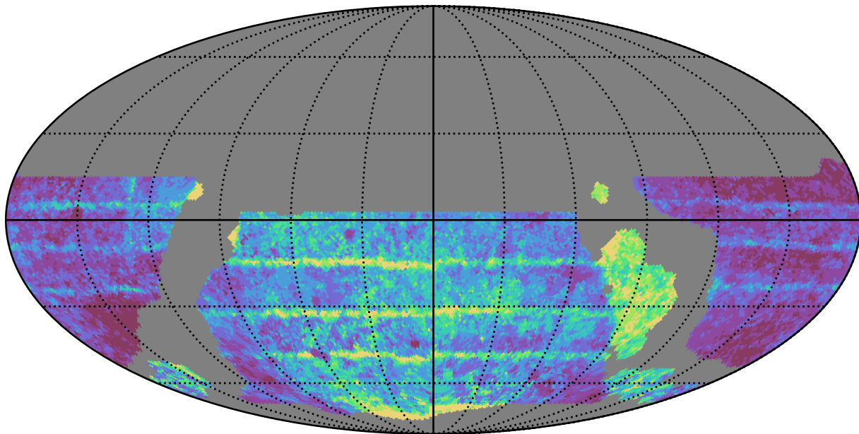
weather_cloudso14v3.4_10yrs WFD z band: Median Inter-Night Gap
