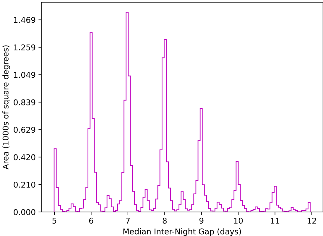
weather_cloudso14v3.4_10yrs WFD z band: Median Inter-Night Gap
