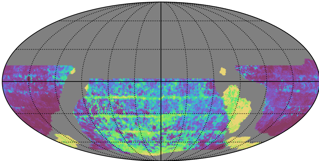
weather_cloudso14v3.4_10yrs WFD y band: Median Inter-Night Gap
