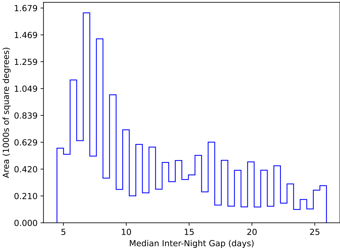
weather_cloudso14v3.4_10yrs WFD y band: Median Inter-Night Gap
