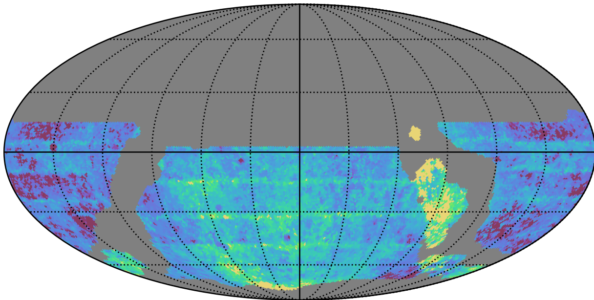
weather_cloudso14v3.4_10yrs WFD u band: Median Inter-Night Gap
