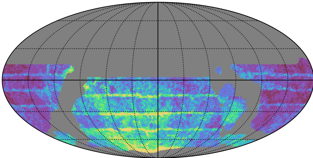
weather_cloudso14v3.4_10yrs WFD r band: Median Inter-Night Gap
