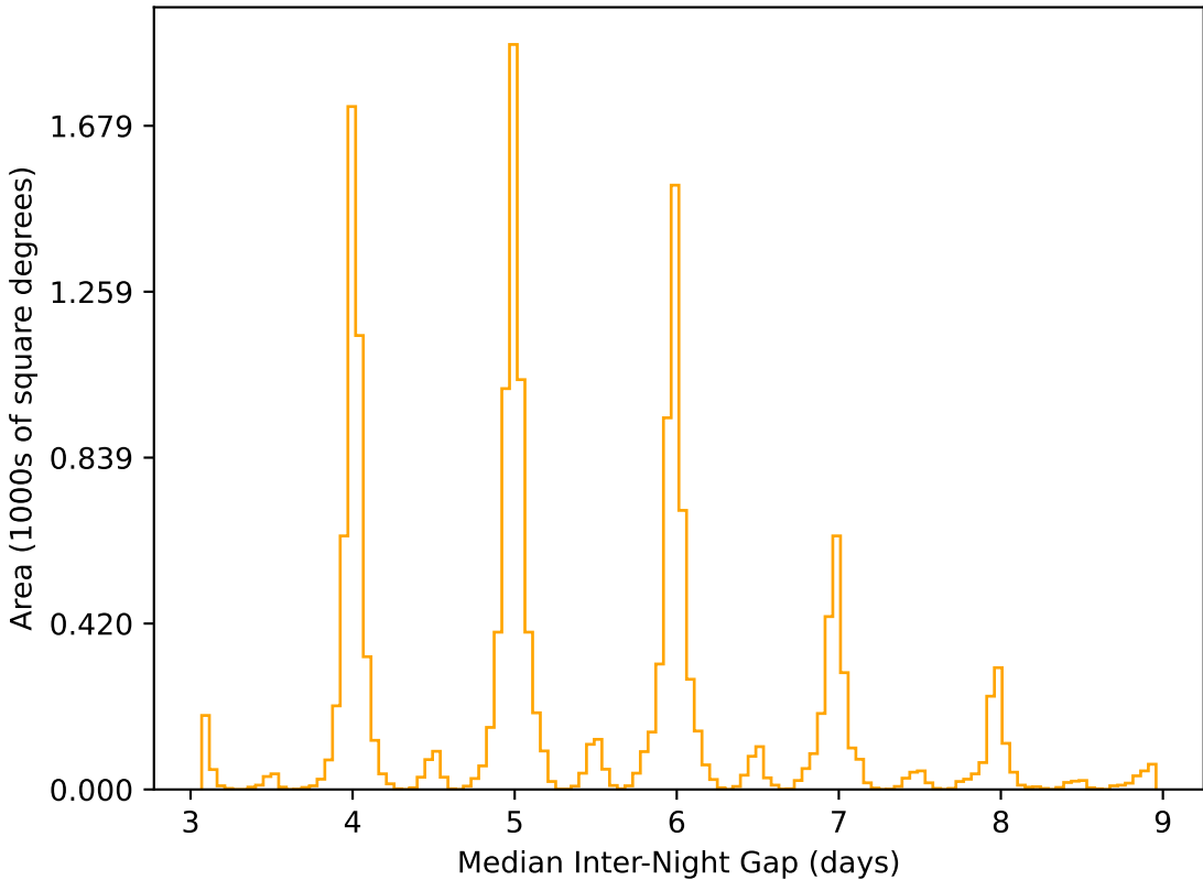
weather_cloudso14v3.4_10yrs WFD r band: Median Inter-Night Gap
