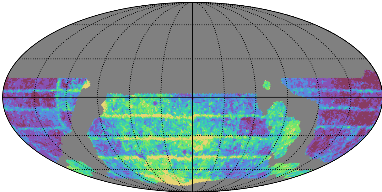
weather_cloudso14v3.4_10yrs WFD i band: Median Inter-Night Gap
