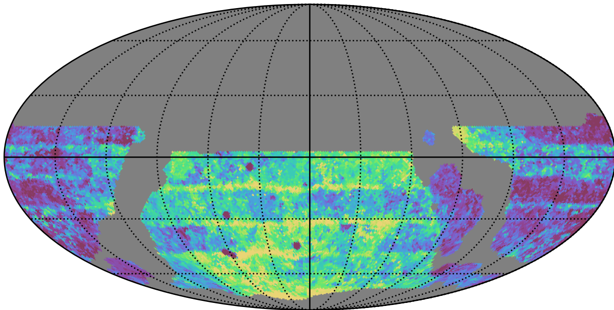
weather_cloudso14v3.4_10yrs WFD g band: Median Inter-Night Gap
