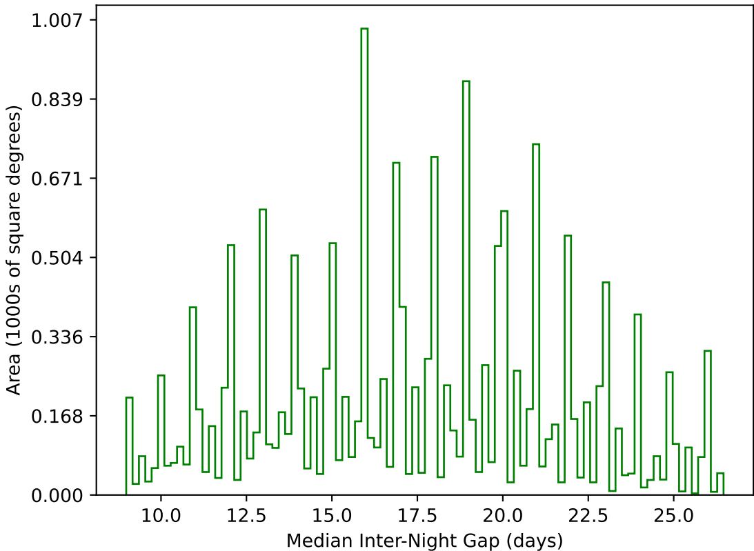
weather_cloudso14v3.4_10yrs WFD g band: Median Inter-Night Gap
