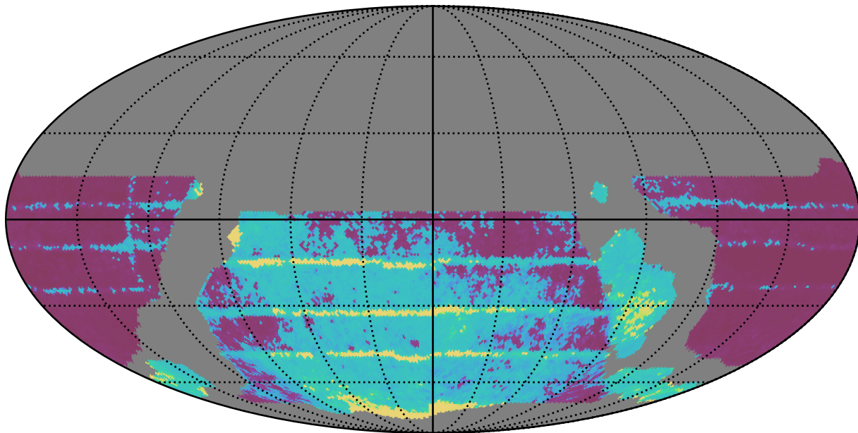
weather_cloudso14v3.4_10yrs WFD all bands: Median Inter-Night Gap
