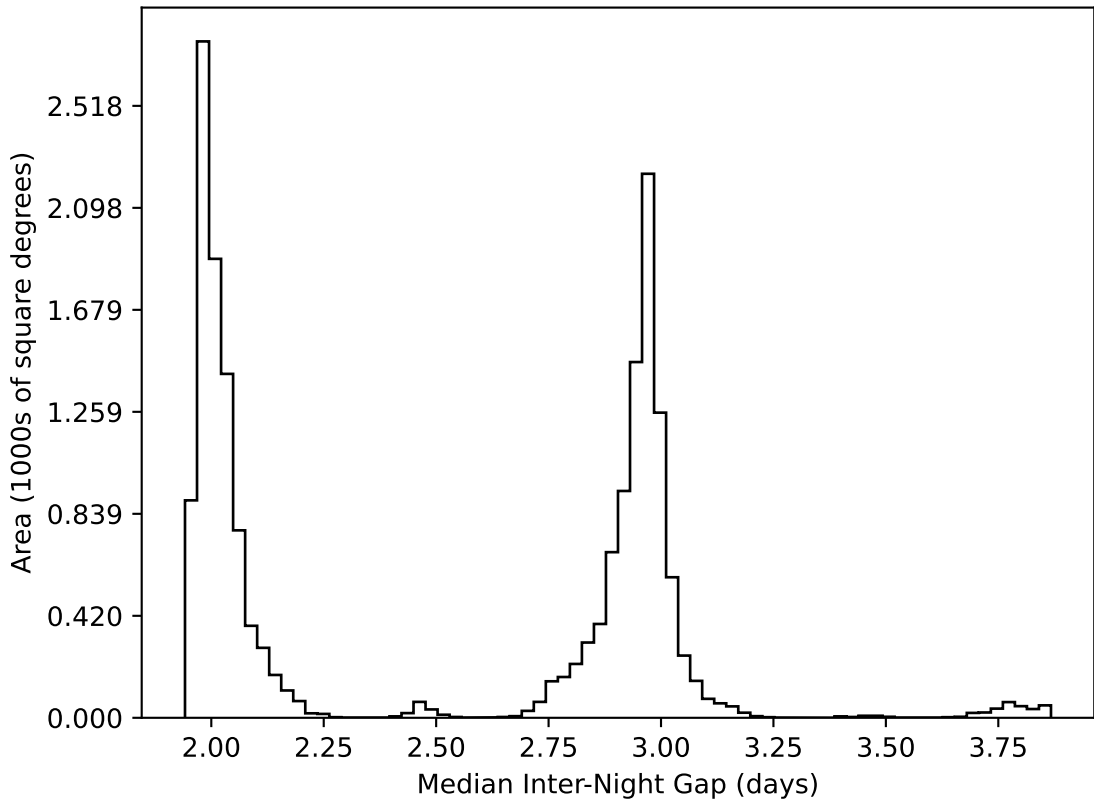
weather_cloudso14v3.4_10yrs WFD all bands: Median Inter-Night Gap
