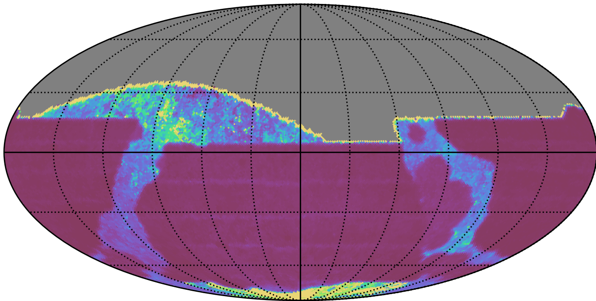
weather_cloudso14v3.4_10yrs All sky z band: Median Inter-Night Gap
