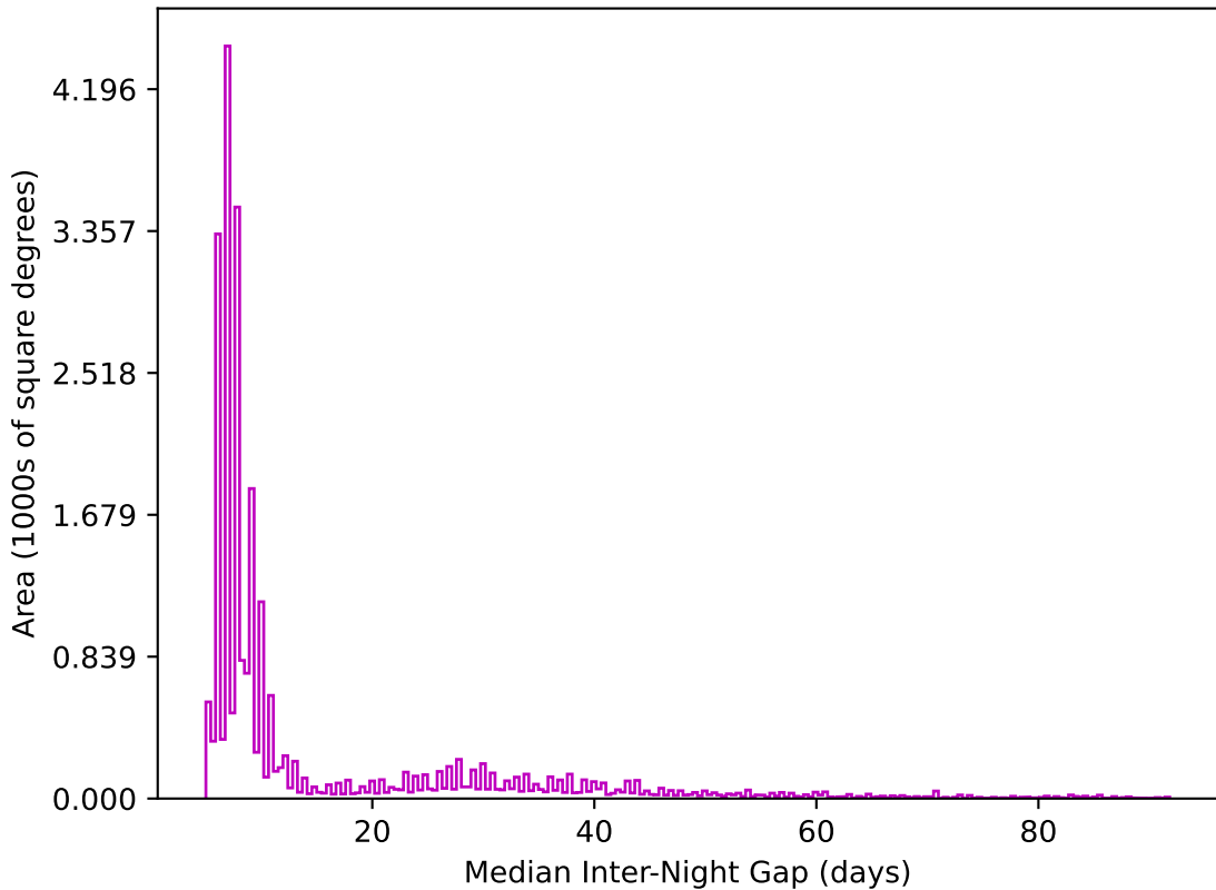
weather_cloudso14v3.4_10yrs All sky z band: Median Inter-Night Gap
