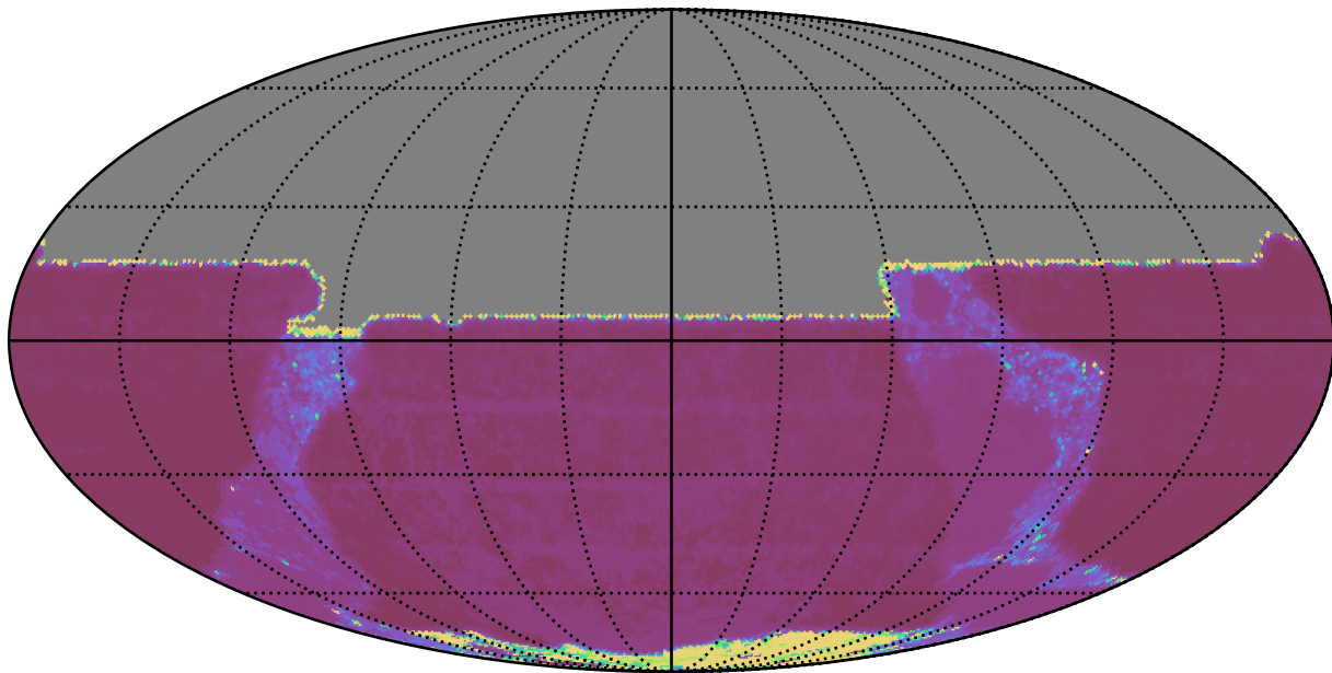
weather_cloudso14v3.4_10yrs All sky y band: Median Inter-Night Gap
