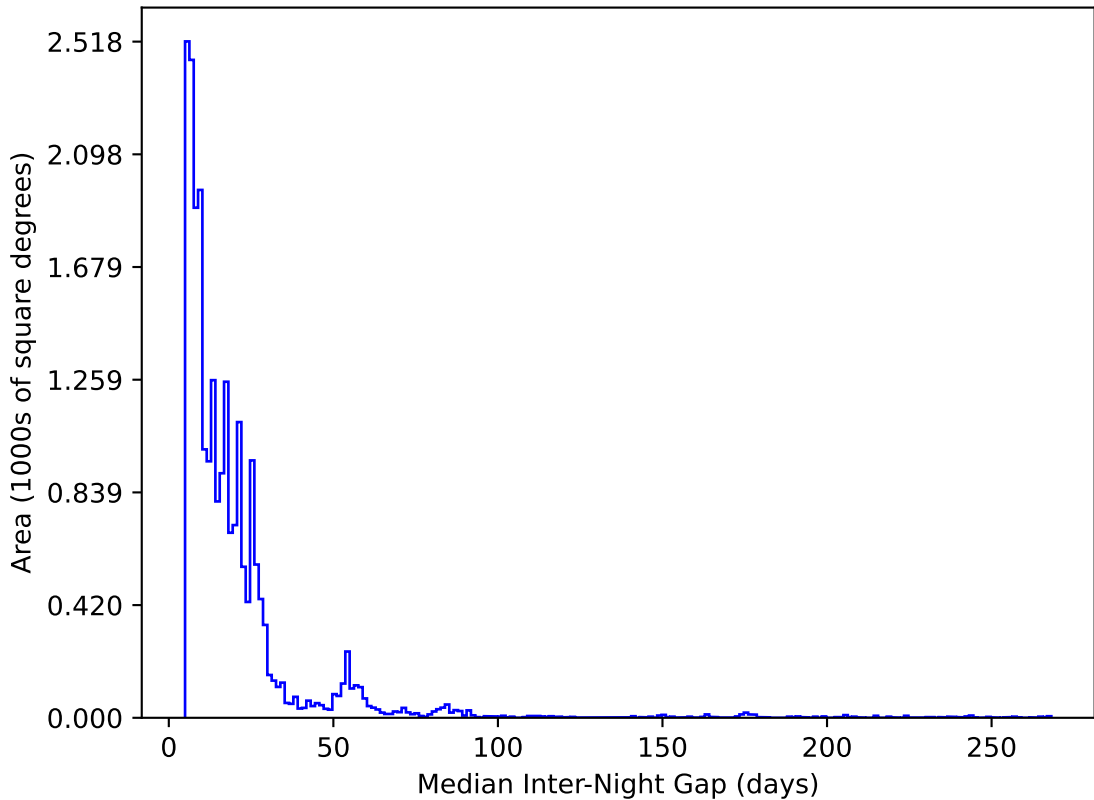
weather_cloudso14v3.4_10yrs All sky y band: Median Inter-Night Gap
