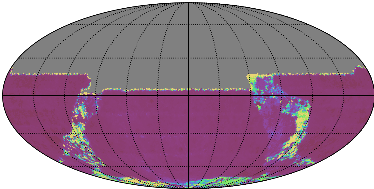
weather_cloudso14v3.4_10yrs All sky u band: Median Inter-Night Gap
