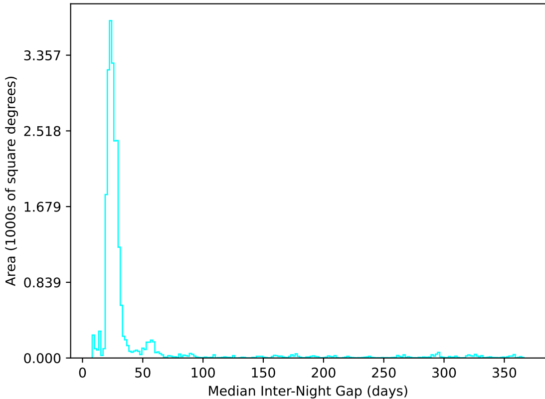
weather_cloudso14v3.4_10yrs All sky u band: Median Inter-Night Gap
