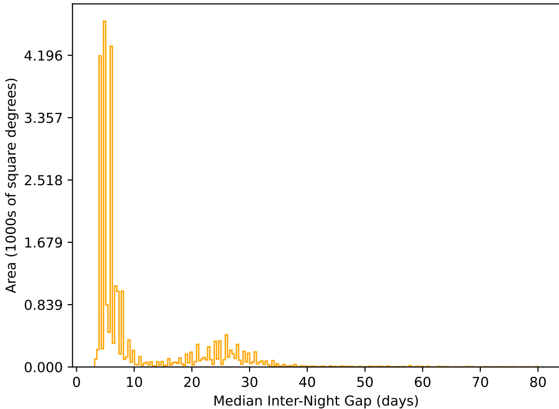
weather_cloudso14v3.4_10yrs All sky r band: Median Inter-Night Gap
