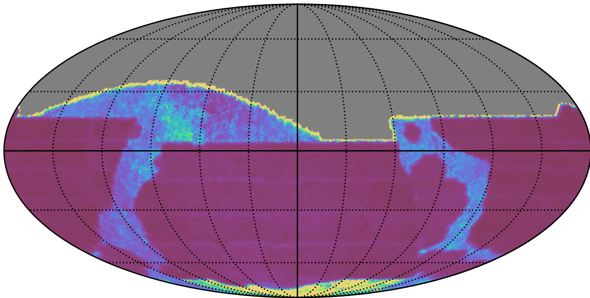
weather_cloudso14v3.4_10yrs All sky i band: Median Inter-Night Gap
