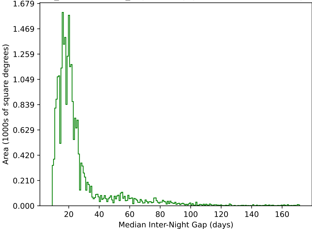
weather_cloudso14v3.4_10yrs All sky g band: Median Inter-Night Gap
