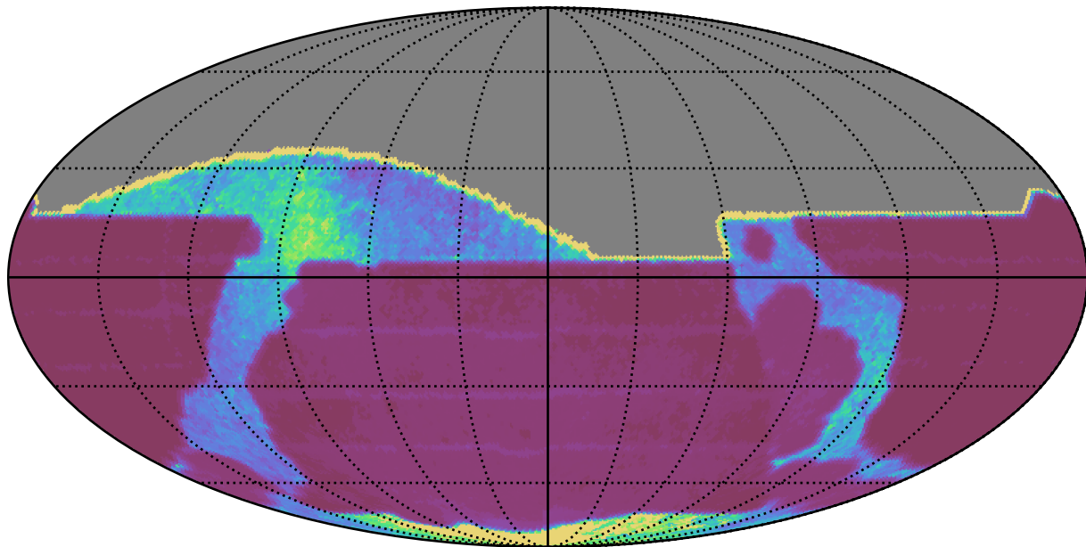
weather_cloudso14v3.4_10yrs All sky all bands: Median Inter-Night Gap
