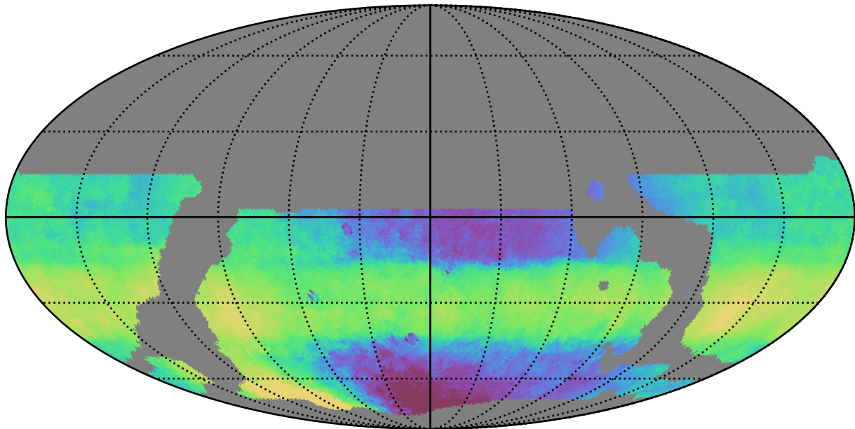
weather_cloudso14v3.4_10yrs WFD z band: Median HA
